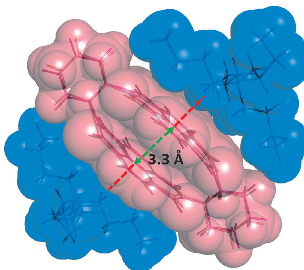
Figure 5. A space-filling representation of the solid-state superstructure of [(-)\text{-2NDI}]^{2-}\cdot 2\text{Bu}_4\text{N}^+ in which the radical anion dimer is illustrated in pink while the two tetrabutylammonium ions are illustrated in blue. A tubular representation (pale pink and dark blue) of the same solid-state structure, which shows the intramolecular \pi - \pi stacking distance between the two \text{NDI}^{\cdot-} radical anions, is superimposed upon the space-filling representation. Note that there are [\text{C}-\text{H}\cdots\pi] interactions between the \text{NDI}^{\cdot-} radical anions and the \text{Bu}_4\text{N}^+ cations. The calculated structure (dark pink tubular skeleton) of [(-)\text{-2NDI}]^{2-} is overlaid with the solid-state structure of the cyclophane for comparison.
